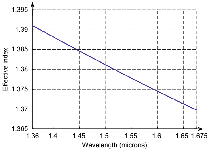
Fig. 7. Effective index curve of the DC-PCF as a function of wavelength. d_1=1 \mu\text{m} , d_2=0.45 \mu\text{m} , d_3=1.35 \mu\text{m} and \Lambda=1.5 \mu\text{m} . n_{\text{silica}}=1.44 and n_{\text{air}}=1 .
